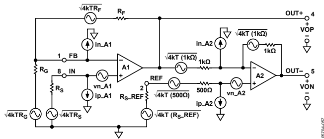
Figure 52. Noise Sources
