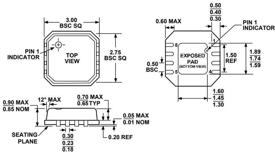
Figure 59. 8-Lead Lead Frame Chip Scale Package [LFCSP_VD] 3 mm x 3 mm Body, Very Thin, Dual Lead (CP-8-2) Dimensions shown in millimeters
